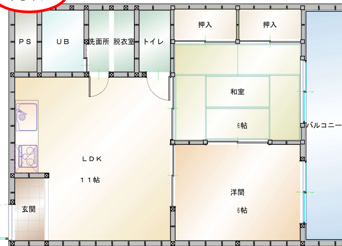
間取
